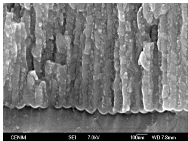
Figure 9. Cross section of the sealed anodized coating in the zone of the barrier layer.
