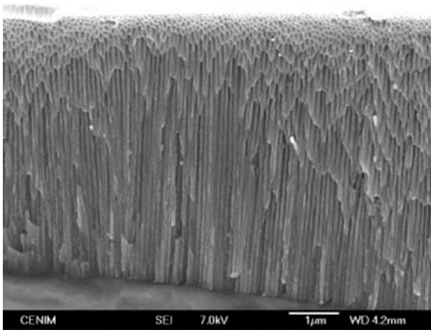
Figure 6. SEM view of cross section obtained by tensile fracture of the unsealed anodic coating showing the tubular form of the pores.
