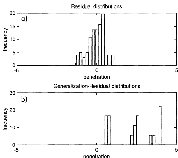
Figure 2. Distribution of the discrepancies between the ANN output and the measurements. a) For the training set, b) for the testing set.
