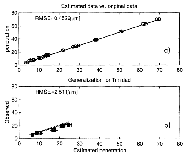
Figure 1. a) Comparison of measured vs. calculated penetration values (in \mu\text{m} ) for the training set. b) The same, for the testing set.
