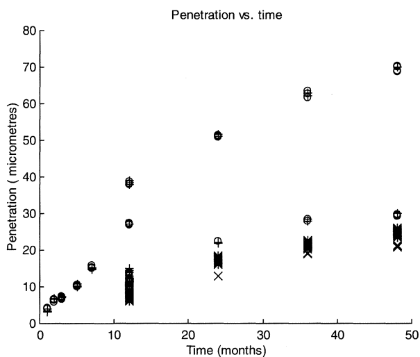
Figure 3. Evolution of the cumulated penetration vs. time of exposure. "o" estimated values and "+" observed values, both for training set. "*" estimated values and "x" observed values both for testing set.
