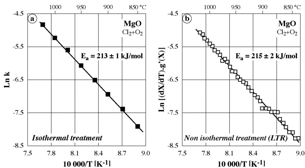
Figure 14. Arrhenius diagram of the MgO oxychlorination by \text{Cl}_2+\text{O}_2 for: (a) isothermal treatment and (b) non isothermal treatment.
