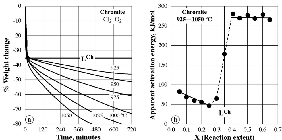
Figure 10. Oxychlorination of chromite between 925 and 1050 °C in \text{Cl}_2+\text{O}_2 atmosphere. (b) Shows the evolution of the apparent activation energy values as a function of the reaction extent calculated from the data of (a).
