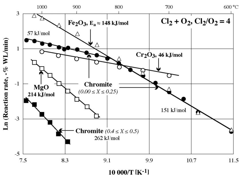
Figure 11. Arrhenius diagrams for the oxychlorination of chromite and its simple oxides in \text{Cl}_2+\text{O}_2 .
